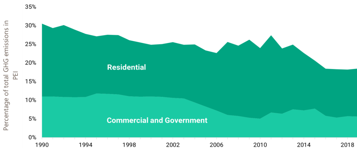
Figure 9: Building emissions decreased to 18% of total GHG emissions in 2018.
