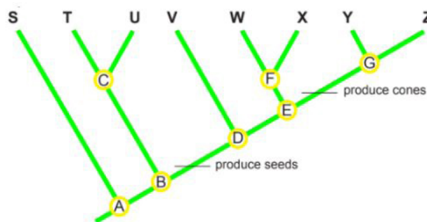
Figure 14. Evolutionary Tree
